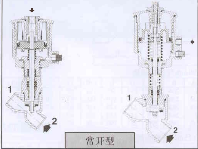
50mm 气控头
