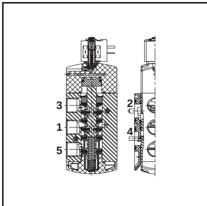
monostable 552 - 553 series
